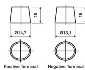
T3 Small Japanese JIS Terminal
