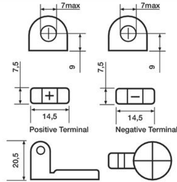
T8 Ford Cargo Terminal use adapter kit (order 23292114)
