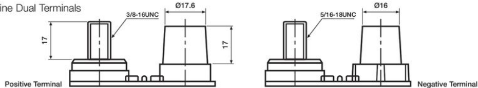
TM Marine Dual Terminals
