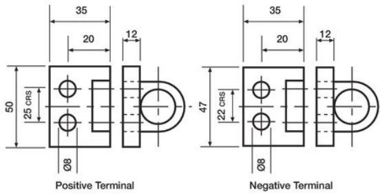
TM Marine Dual Terminals
